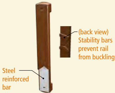
CenFlex® One-Piece Line Bracket
