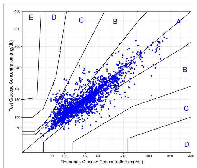
Figure 2. Consensus error grid for the full set of 2,379 pairs of noninvasive/reference measurements.
